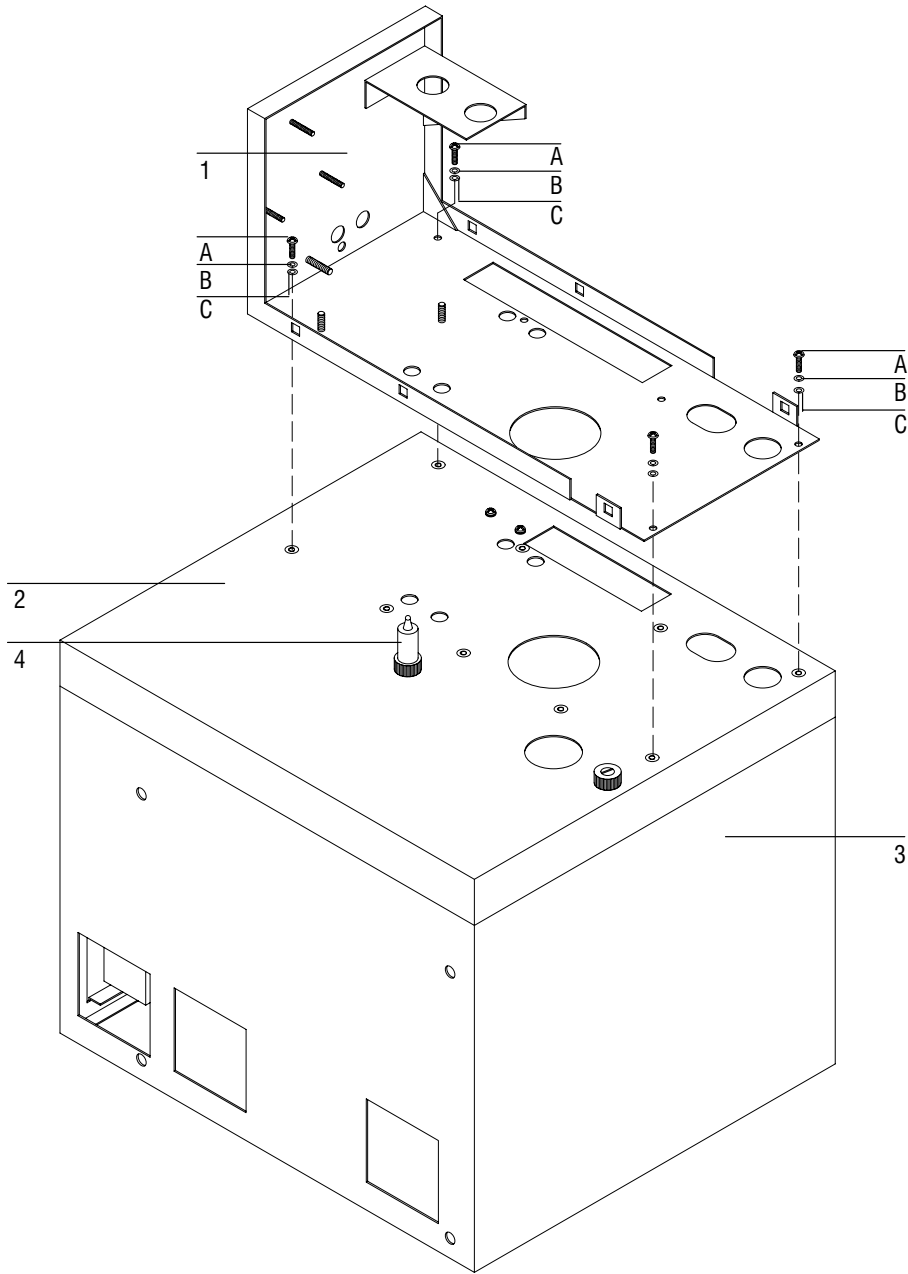
Figure 5-11. Housing
